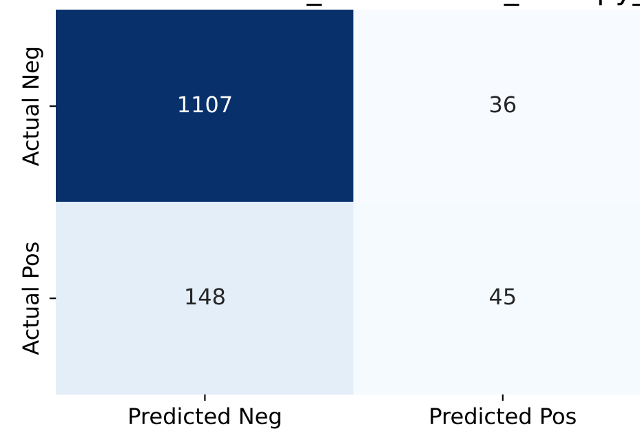
V3-PPO-thresholded_involvement_entropy_reg
