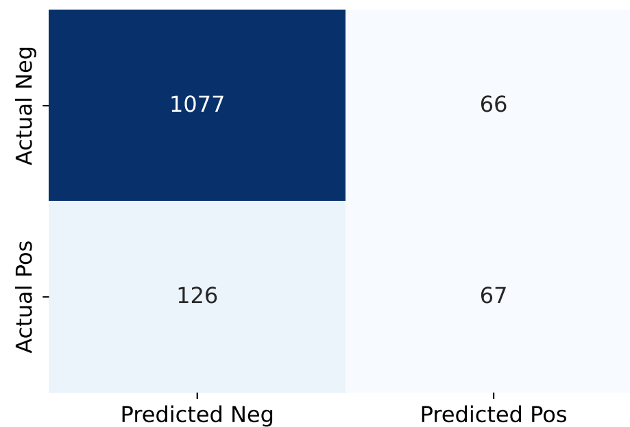
V3-DRPO-continuous-noise-0.3
