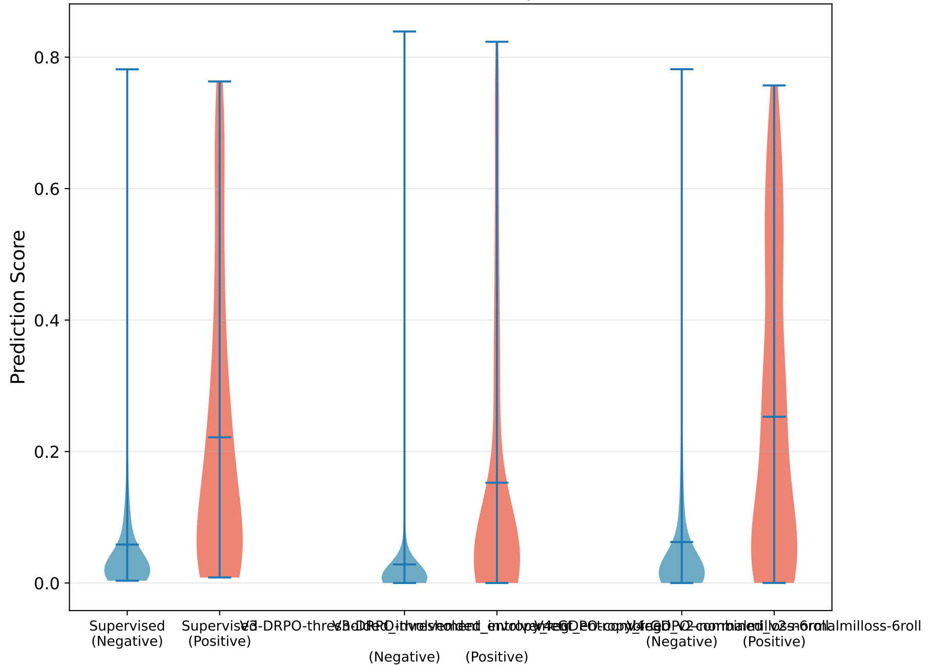
Score Distributions by Class
