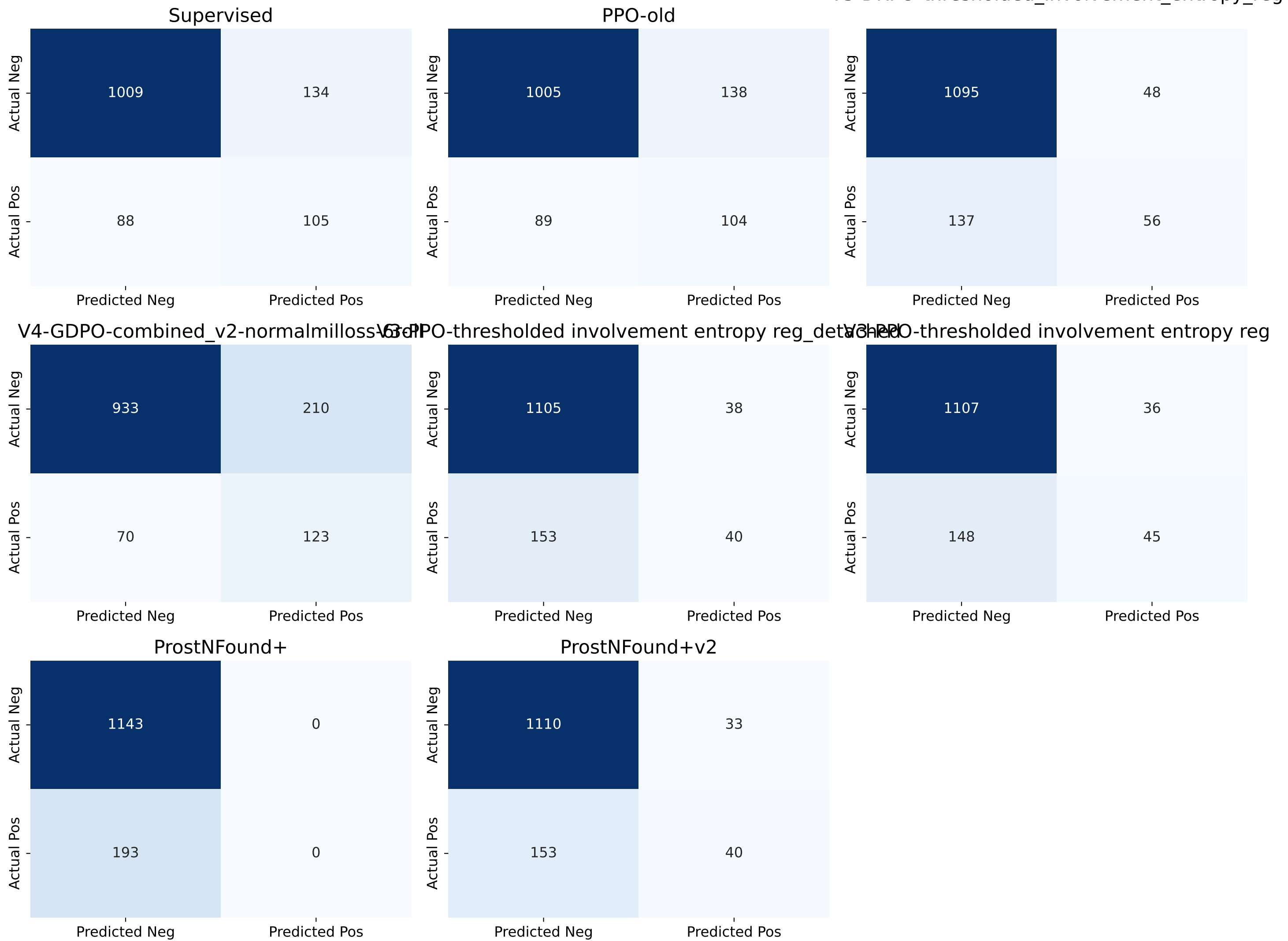
Confusion Matrices at threshold=0.5
