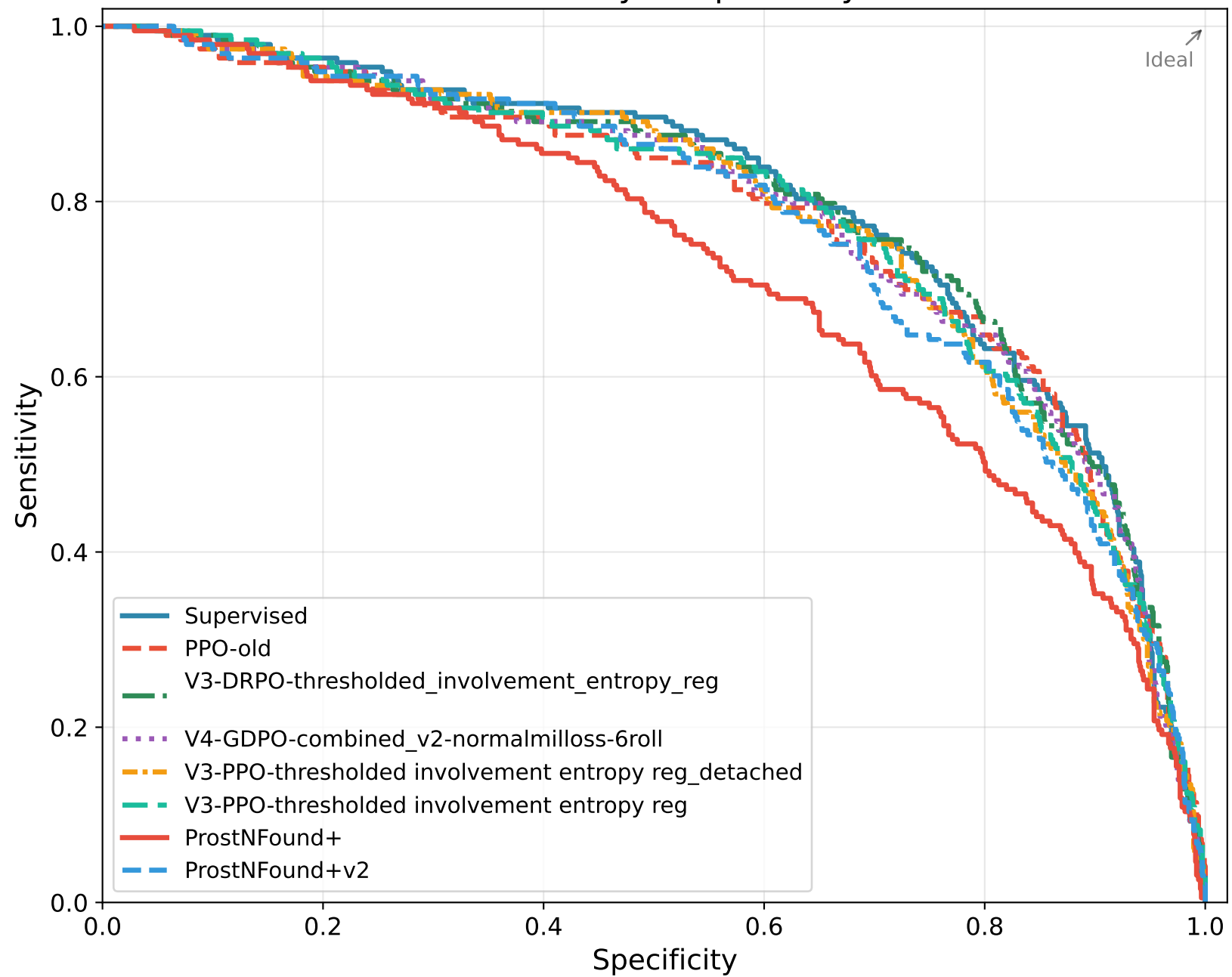
Sensitivity vs Specificity
