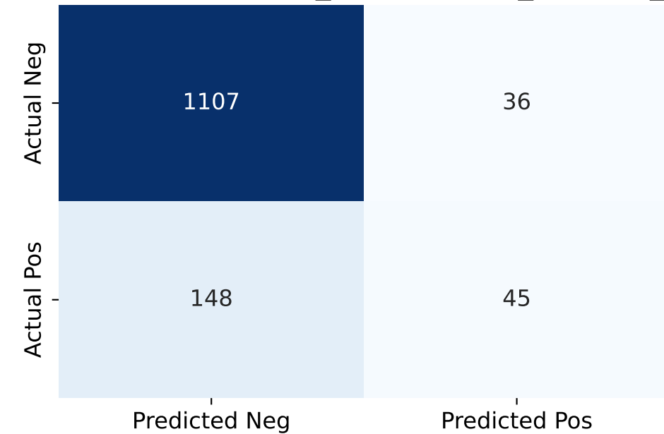
V3-PPO-thresholded_involvement_entropy_reg
