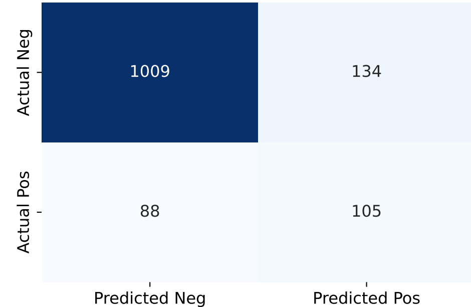
V3-PPO-thresholded_involvement_entropy_reg
