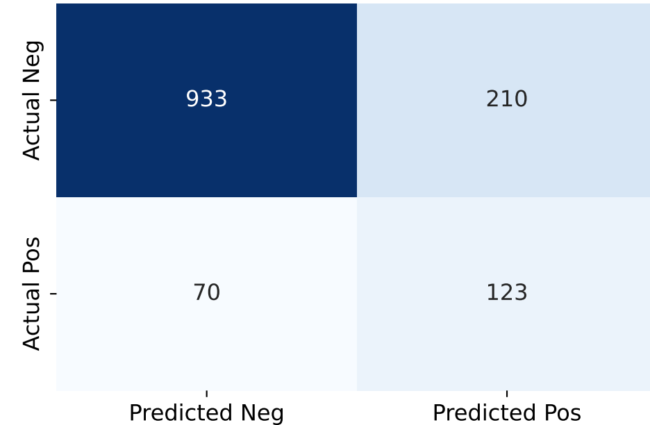
V4-GDPO-combined_v2-normalmilloss-6roll
