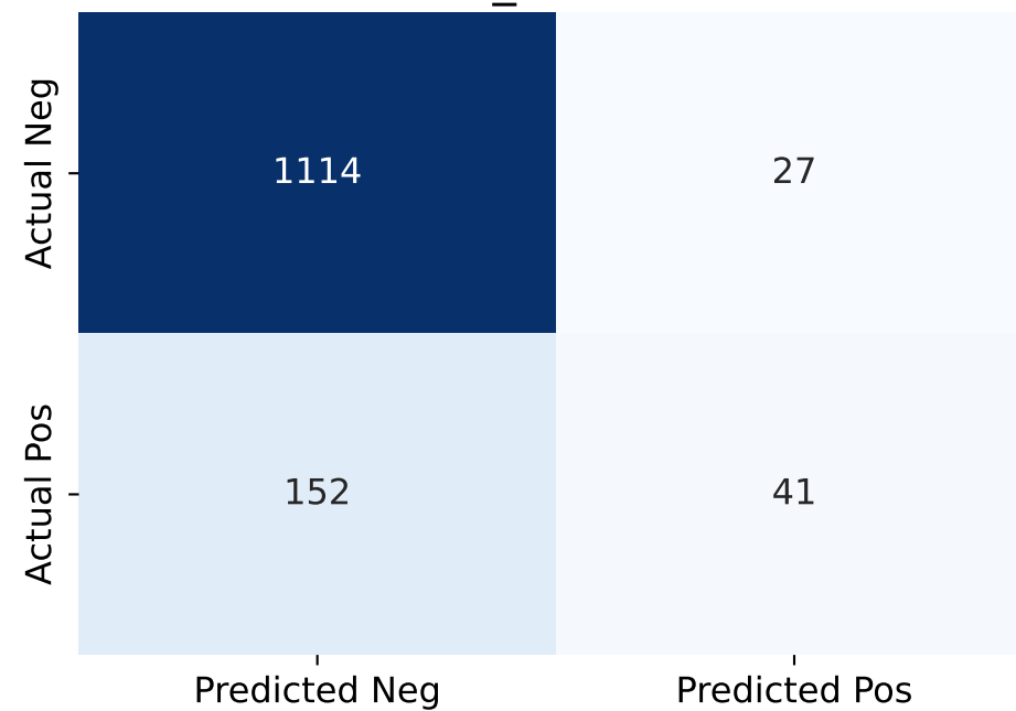
roi_reward
