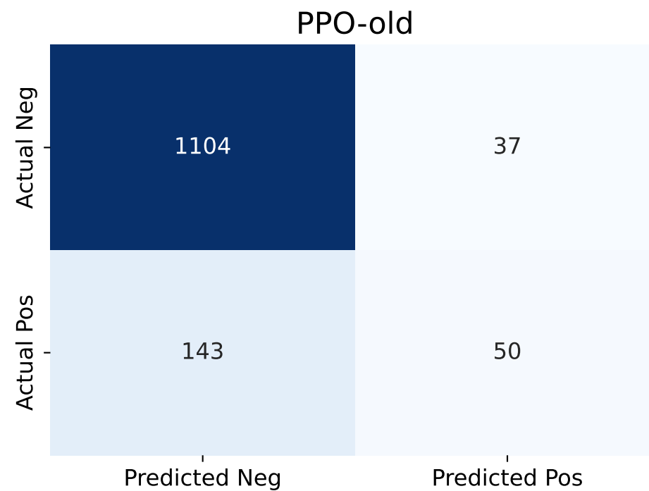
Confusion Matrices at threshold=0.5
