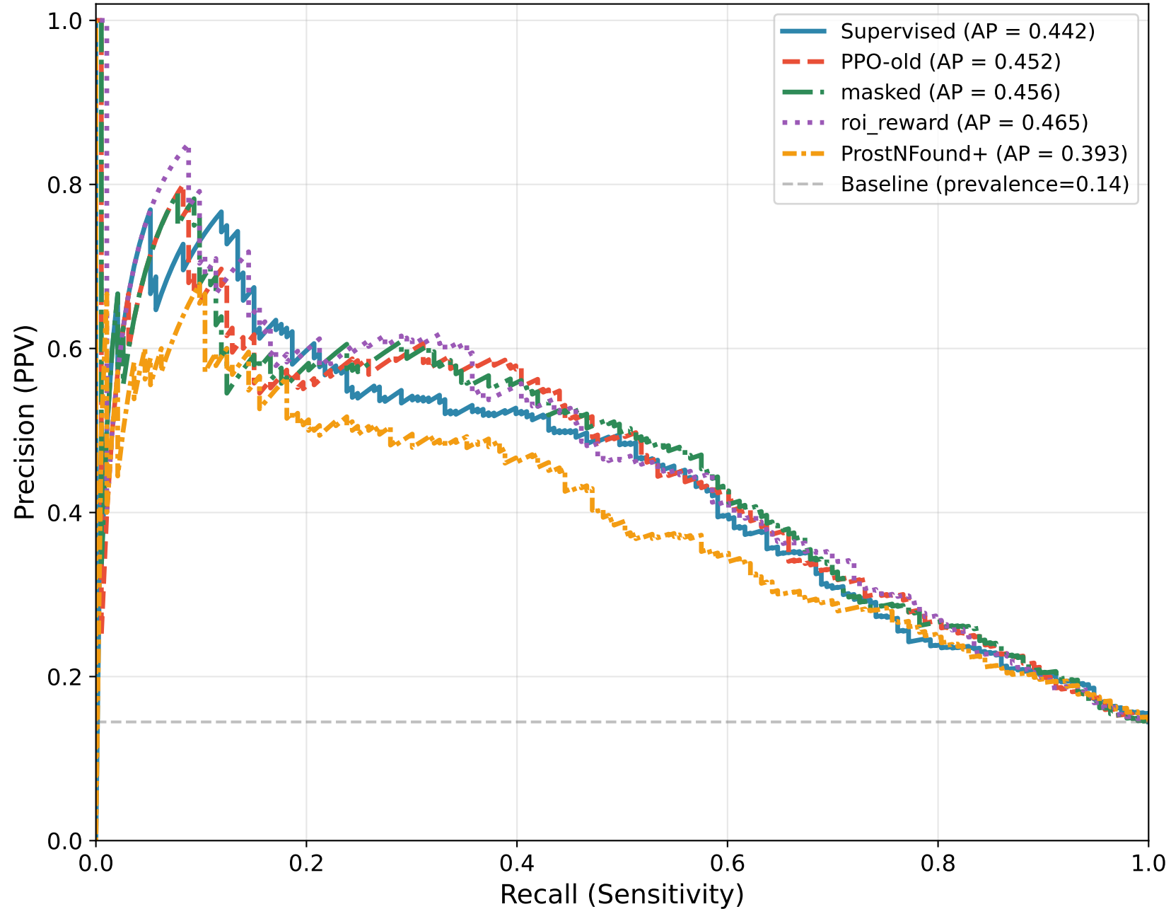
Precision-Recall Curve Comparison
