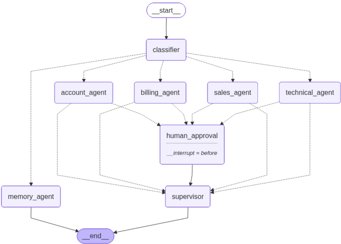
Figure 2.1 - LangGraph workflow architecture diagram.
