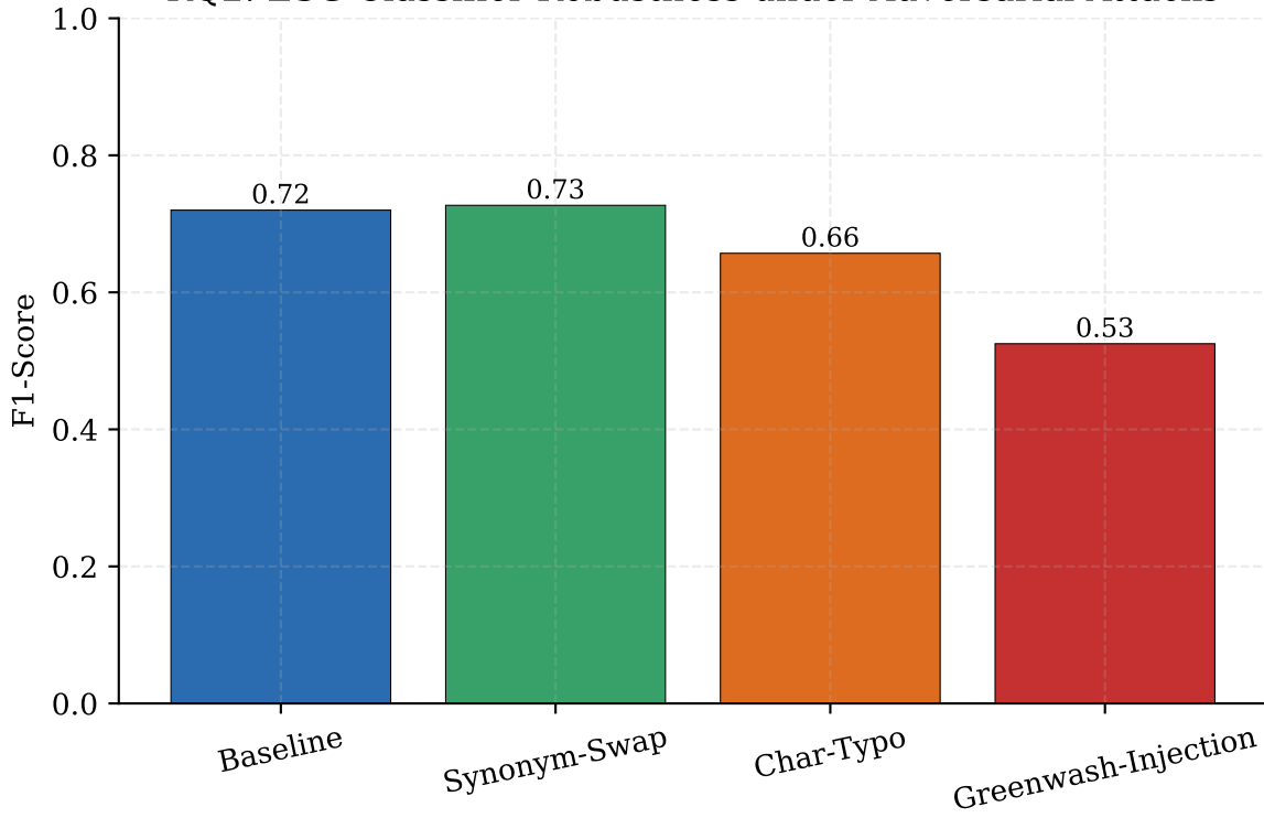
RQ2: ESG Classifier Robustness under Adversarial Attacks
