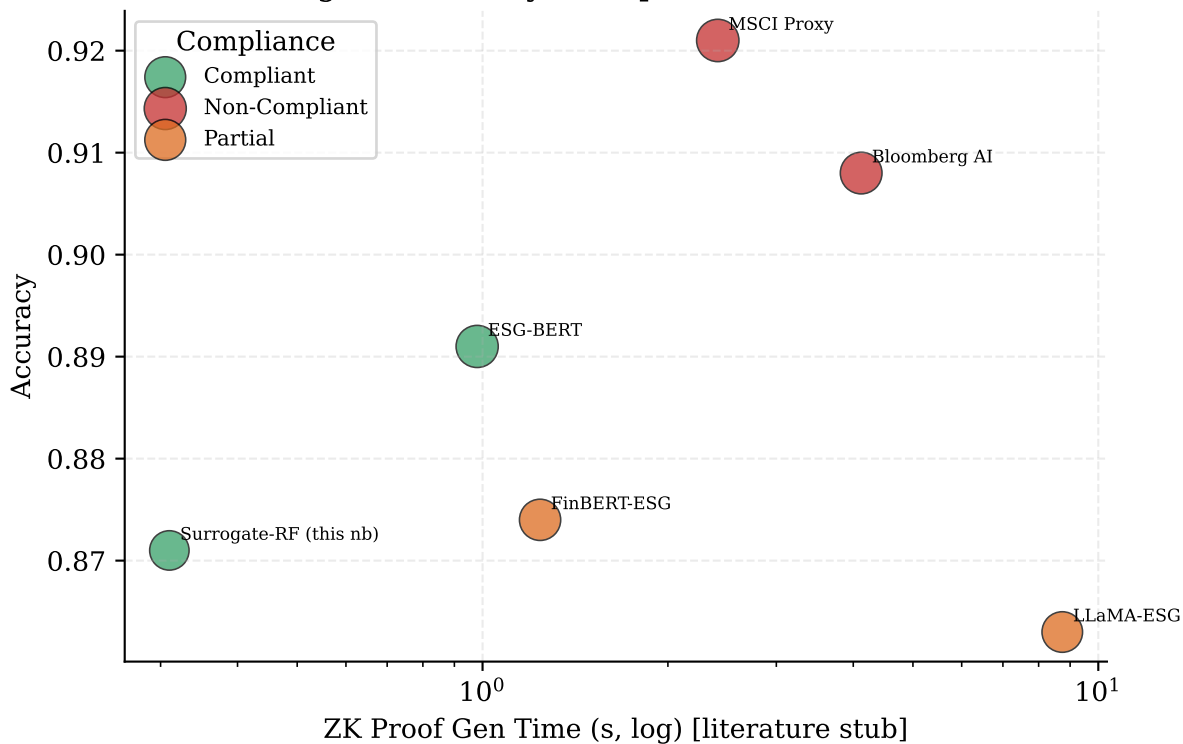
RQ3: Accuracy vs ZK-Proof Cost (surrogate accuracy real; proof times = lit stubs)
