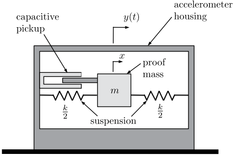
Figure 7.1 Conceptual depiction of MEMS accelerometer.
