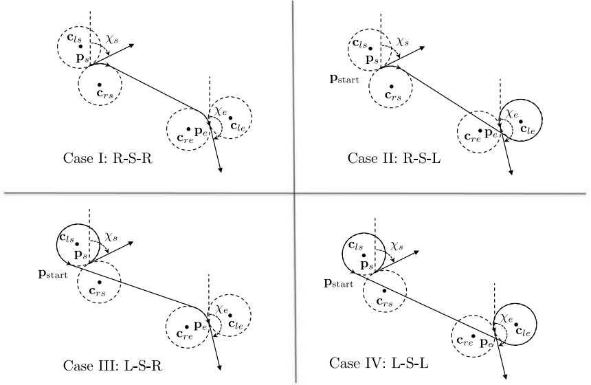
Figure 11.7 Given a start configuration (\mathbf{p}_s, \chi_s) , an end configuration (\mathbf{p}_e, \chi_e) , and a radius R , there are four possible paths consisting of an arc, a straight line, and an arc. The Dubins path is defined as the case that results in the shortest path length, which for this scenario is Case I.
