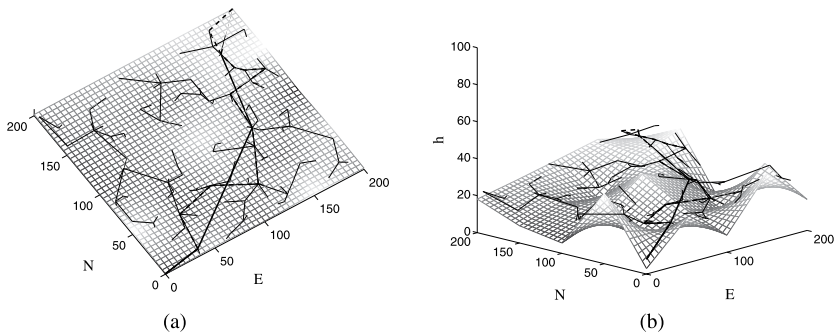
Figure 12.10 (a) Overhead view of the results of the 3-D RRT waypoint path planning algorithm. (b) Side view of the results of the 3-D RRT waypoint path planning algorithm. The thin lines are the RRT graph, the thick dashed line is the RRT path returned by algorithm 10, and the thick solid line is the smoothed path. The RRT graph is generated at a fixed height above the terrain.
