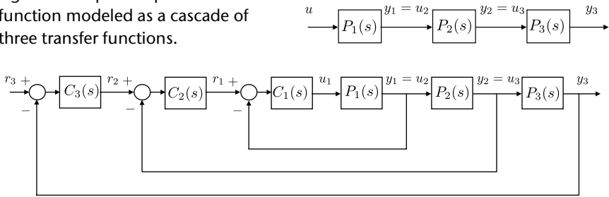
Figure 6.2 Three-stage successive loop closure design.
