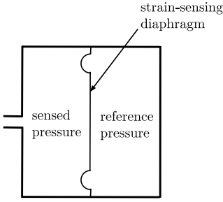
Figure 7.4 Schematic of an absolute pressure sensor.
