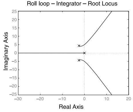
Figure 6.10 Roll loop root locus as a function of the integral gain k_{i_\phi} .
