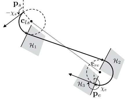
Figure 11.13 Definition of switching half planes for Dubins paths. The algorithm begins in a circular orbit and switches to straight-line tracking when \mathcal{H}_1 is entered. Orbit tracking is again initialized upon entering \mathcal{H}_2 . The half plane \mathcal{H}_3 defines the end of the Dubins path.
