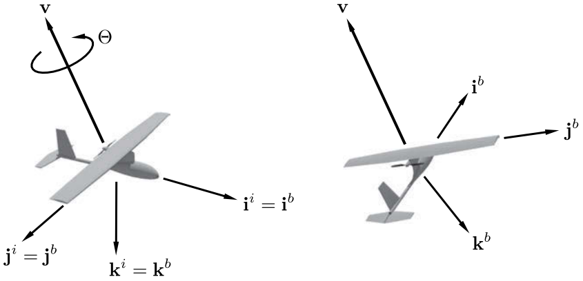
Figure B.1 Rotation represented by a unit quaternion. The aircraft on the left is shown with the body axes aligned with the inertial frame axes. The aircraft on the right has been rotated about the vector v by \Theta = 86 deg. This particular rotation corresponds to the Euler sequence \psi = -90 deg, \theta = 15 deg, \phi = -30 deg.
