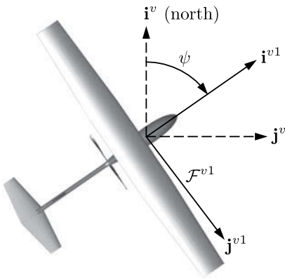
Figure 2.4 The vehicle coordinate frame. The \mathbf{i}^v -axis points north, the \mathbf{j}^v -axis points east, and the \mathbf{k}^v -axis points into the earth.
