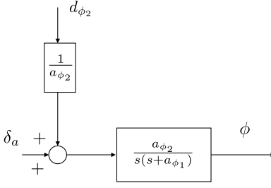
Figure 5.2 Block diagram for roll dynamics. The inputs are the ailerons \delta_a and the disturbance d_{\phi_2} .
