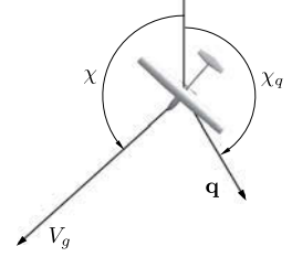
Figure 10.5 The calculation of \chi_q needs to account for the current course angle of the MAV. In this scenario, the MAV should turn left to align with the waypoint path, but if \chi_q is computed with atan2 , the angle will be a positive number slightly smaller than +\pi , which will cause the MAV to turn right to align with the waypoint path.
