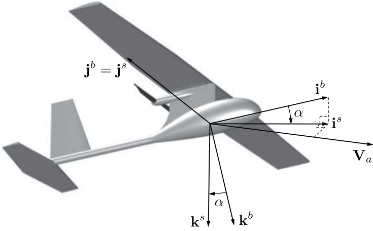
Figure 2.8 The stability frame. The \mathbf{i}^s -axis points along the projection of the airspeed vector onto the \mathbf{i}^b - \mathbf{k}^b plane of the body frame, the \mathbf{j}^s -axis is identical to the \mathbf{j}^b -axis of the body frame, and the \mathbf{k}^s -axis is constructed to make a right-handed coordinate system. Note that the angle of attack is defined as a left-handed rotation about the body \mathbf{j}^b -axis.
