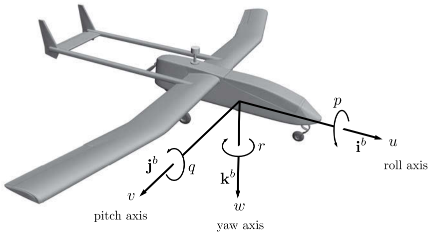
Figure 3.1 Definition of axes of motion.
