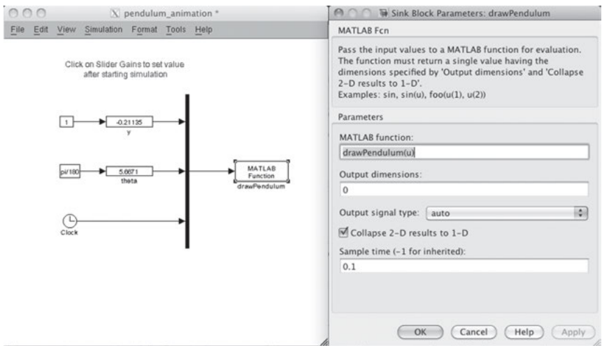
Figure C.2 Simulink file for debugging the pendulum simulation. There are three inputs to the Matlab m-file drawPendulum: the position y , the angle \theta , and the time t . Slider gains for y and \theta are used to verify the animation.
