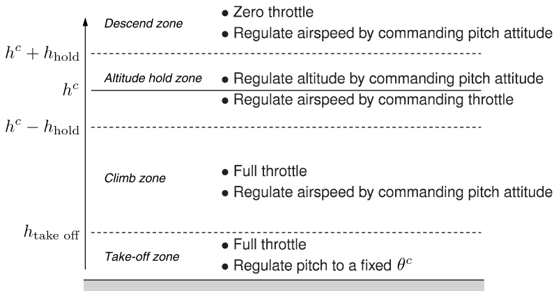
Figure 6.14 Flight regimes for the longitudinal autopilot.
