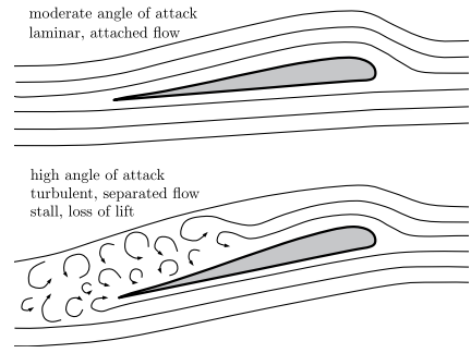
Figure 4.6 The upper drawing depicts a wing under normal flow conditions. The flow is laminar and follows the surface of the wing. The lower drawing shows a wing under stall conditions due to a high angle of attack. In this case, the flow separates from the top surface of the wing, leading to turbulent flow and a significant drop in the lift force produced by the wing.
