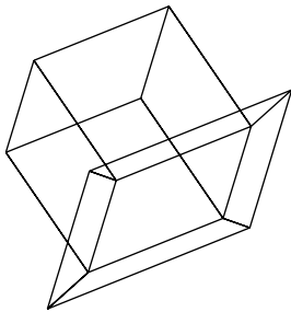
Figure C.4 Rendering of the spacecraft using lines and the plot3 command.
