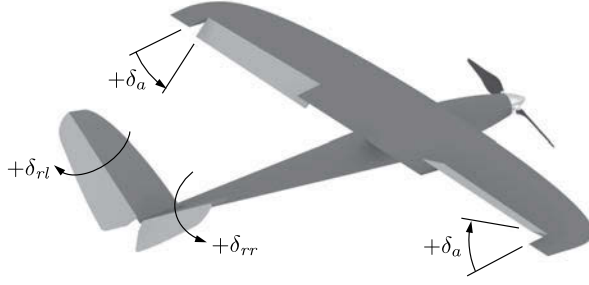
Figure 4.4 Ruddervators are used to control a v-tail aircraft. The ruddervators replace the rudder and the elevator. Driving the ruddervators together has the same effect as an elevator, and driving them differentially has the same effect as a rudder.
