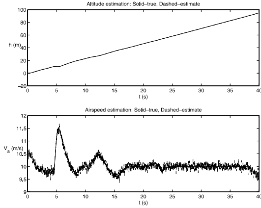
Figure 8.3 Estimation error of the altitude and airspeed obtained by low-pass filtering the pressure sensors and inverting the sensor model. For altitude and airspeed, the accuracy of the simple scheme is adequate.
