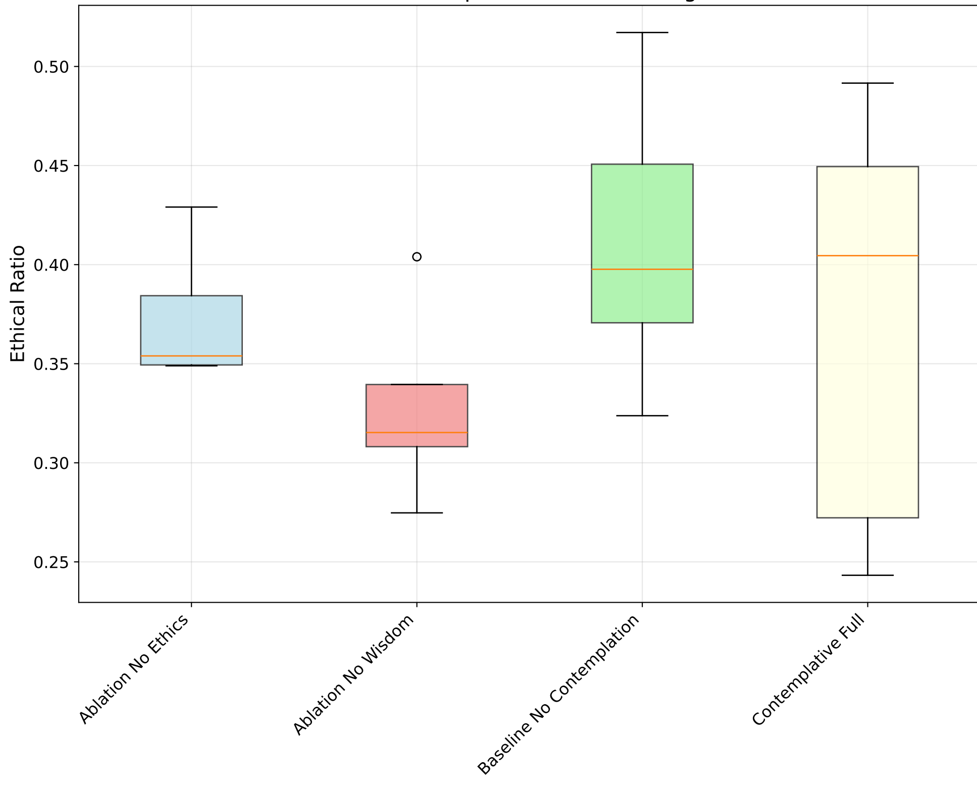
Ethical Ratio Comparison Across Configurations
