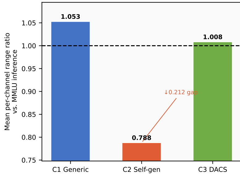
Cybersecurity (Llama 3.1 8B)
