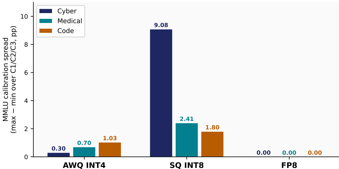
Calibration sensitivity per (format × domain) on MMLU
