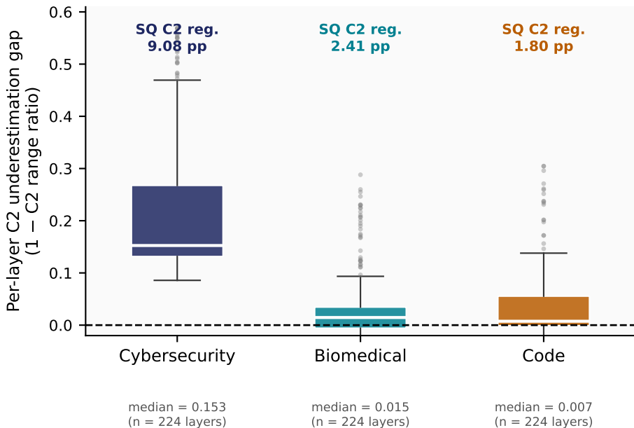
Fig. 6: Per-layer C2 underestimation gap by domain (n = 224 SmoothQuant-targeted layers per box)
