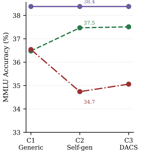
Code (CodeLlama-7B-Instruct)
