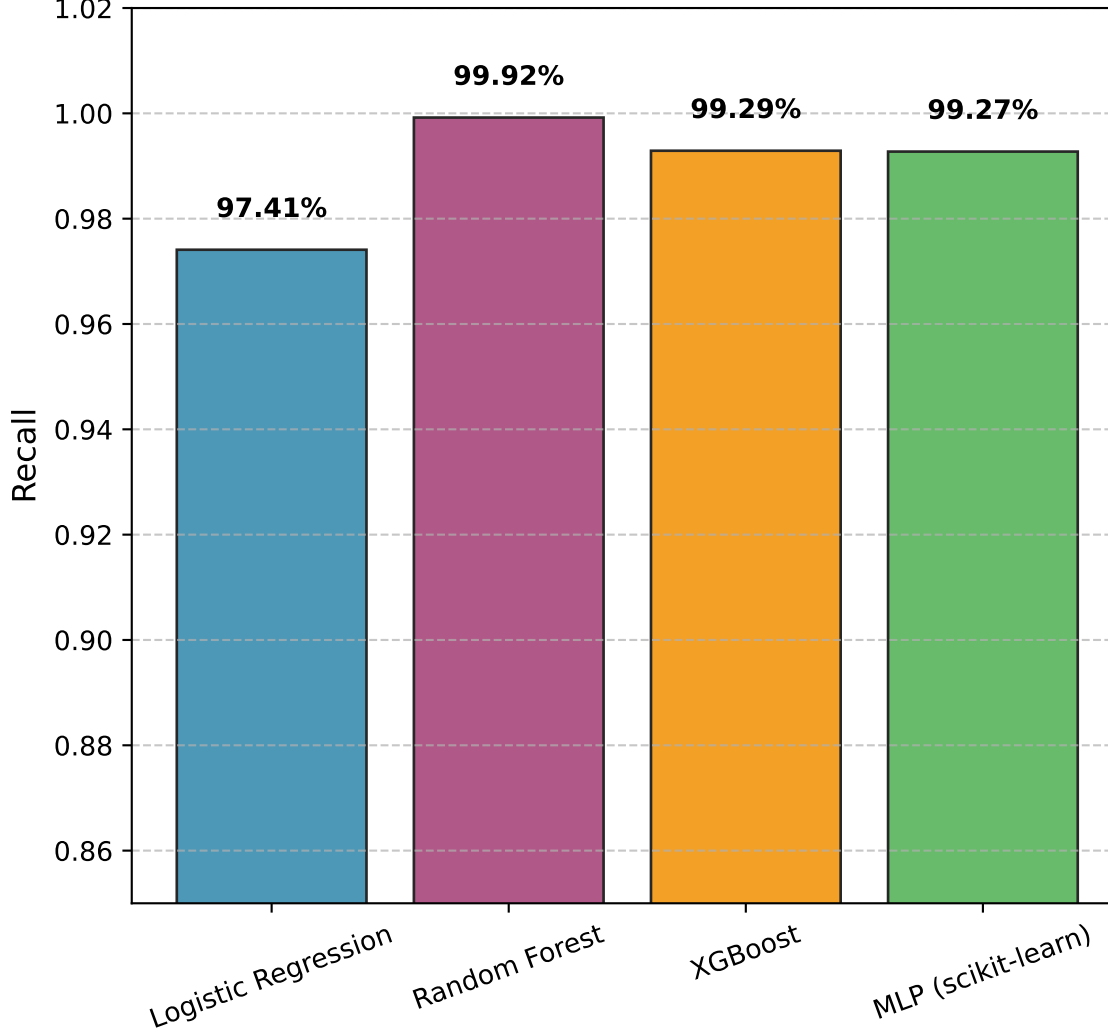
Recall Comparison
