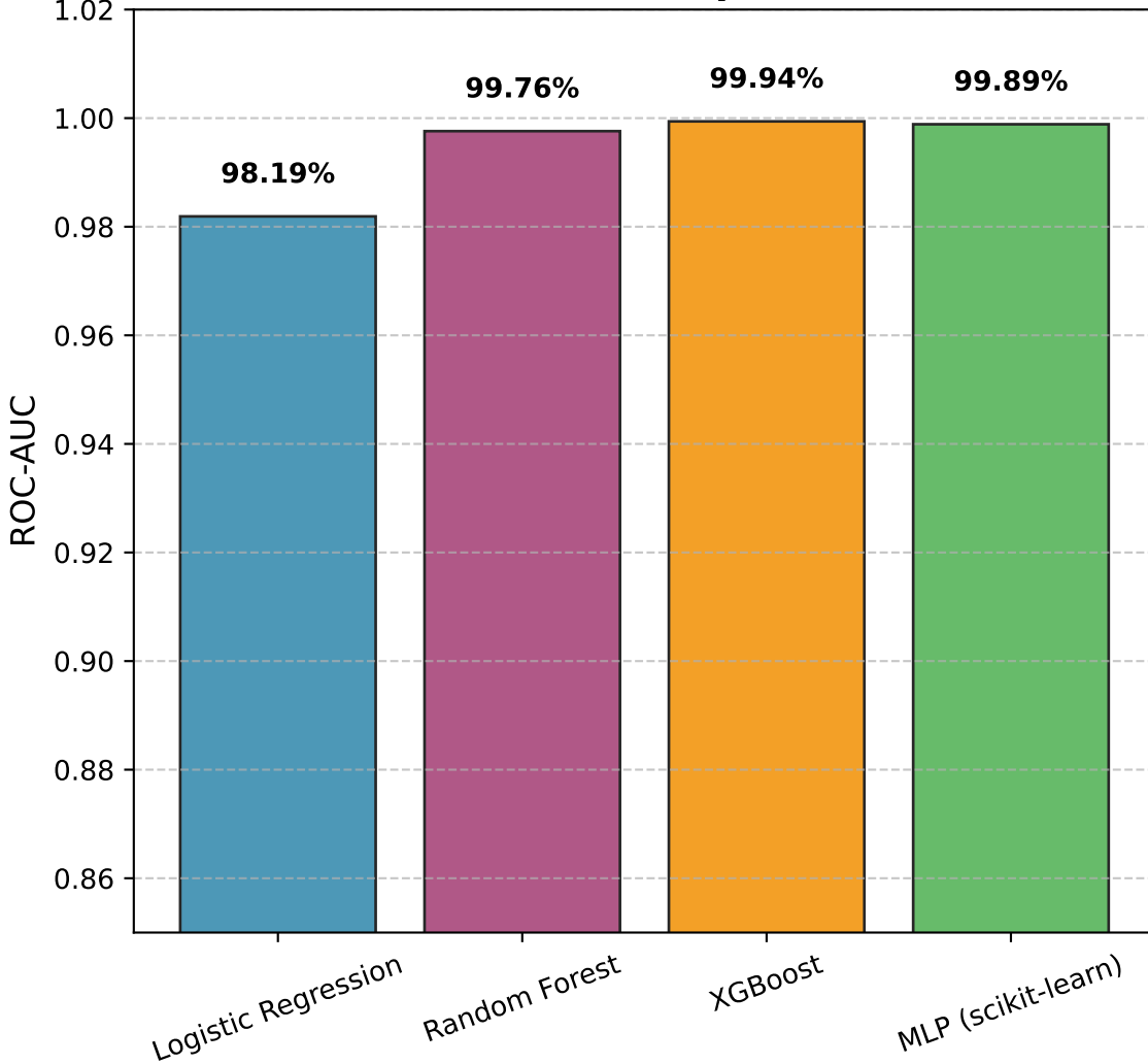
ROC-AUC Comparison
