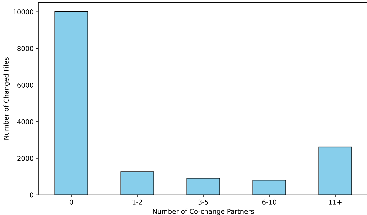
Applicability: Distribution of Partners-per-Changed-File
