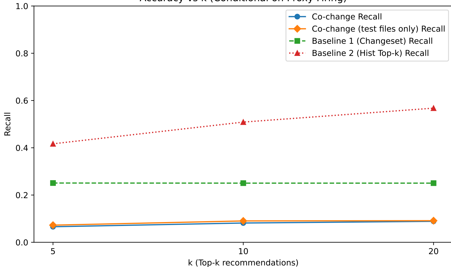
Accuracy vs k (Conditional on Proxy Firing)
