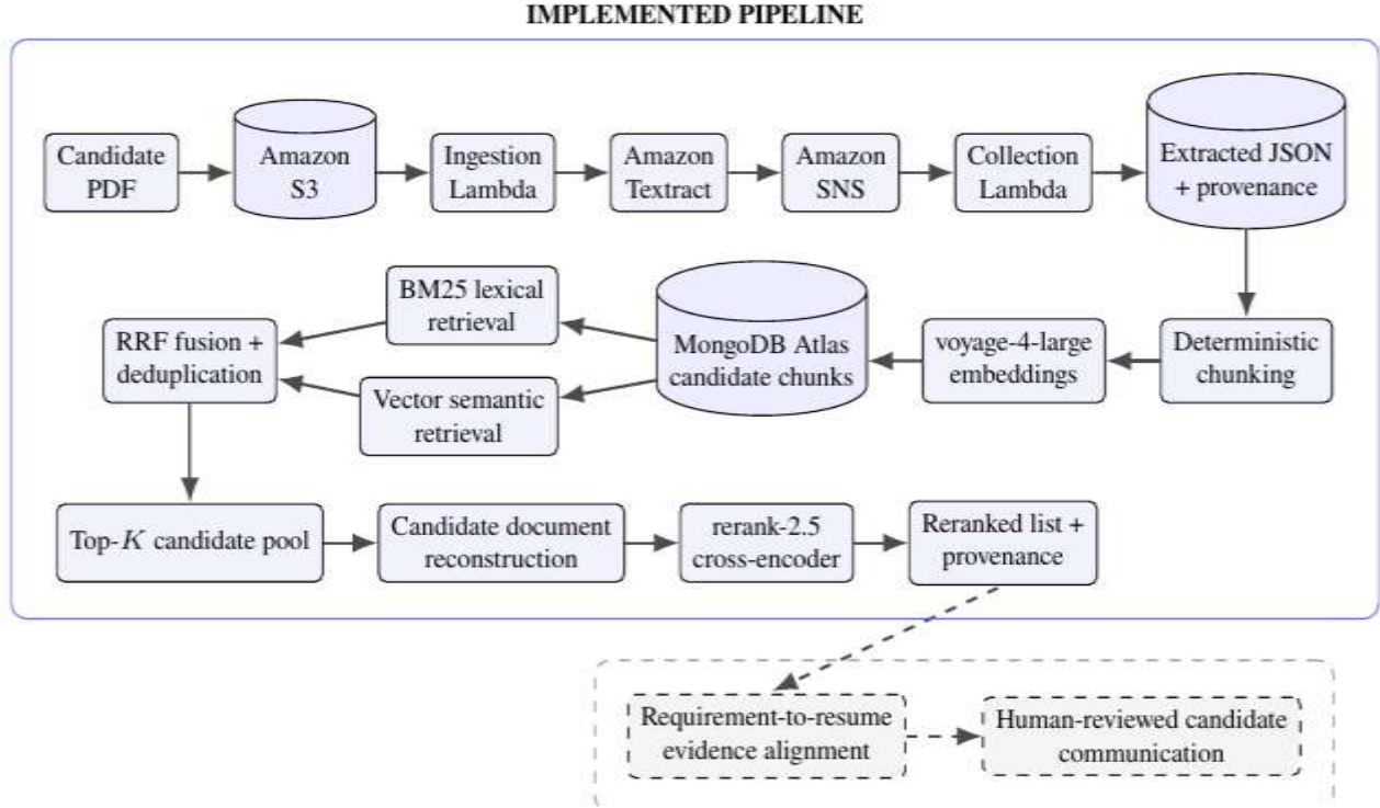
Figure 2. Hybrid retrieval and cross-encoder reranking pipeline with proposed evidence and communication extensions.
