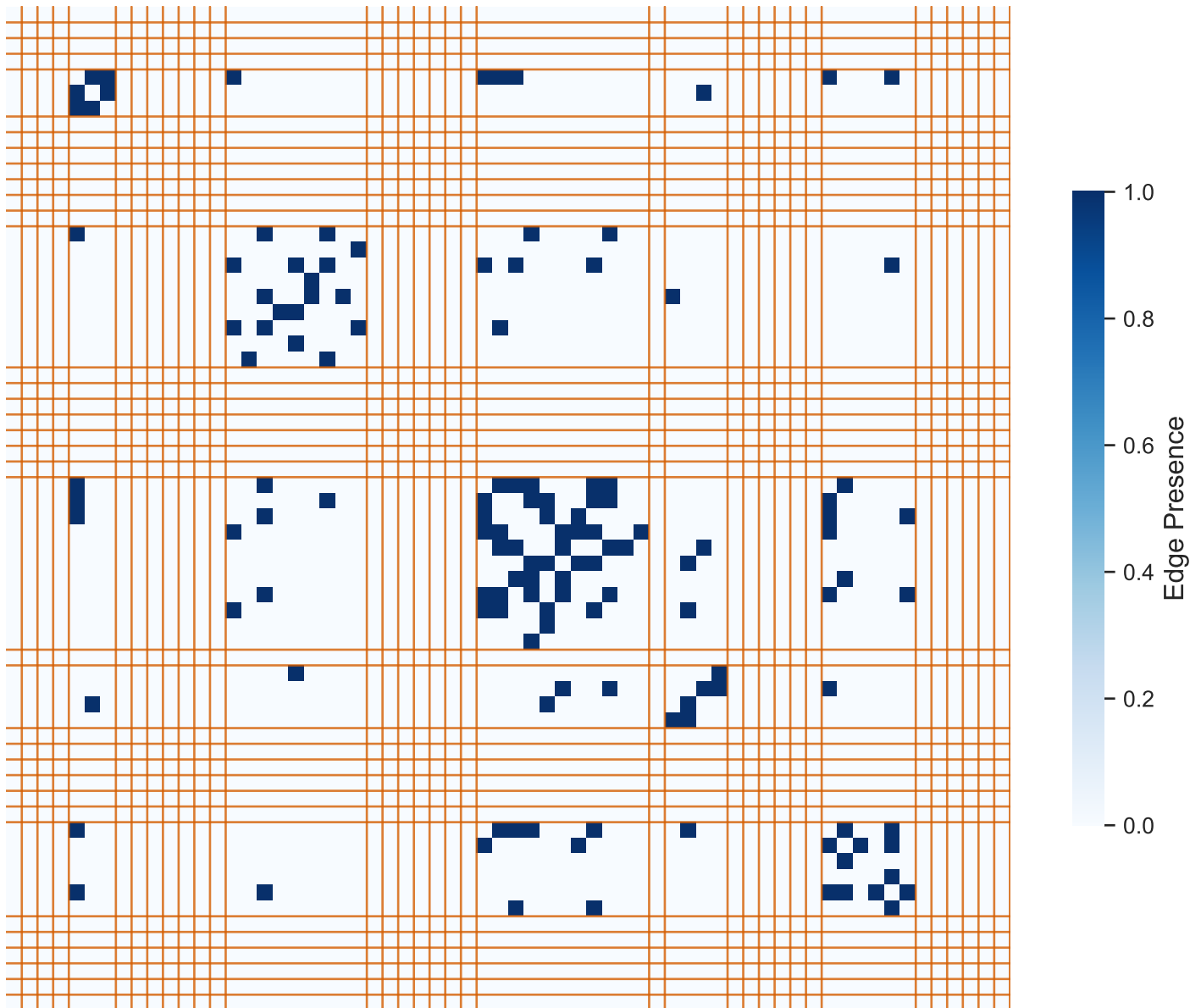
Block Adjacency — Aggregated Layer ( k = 8 ) (Rows/Cols sorted by community)
