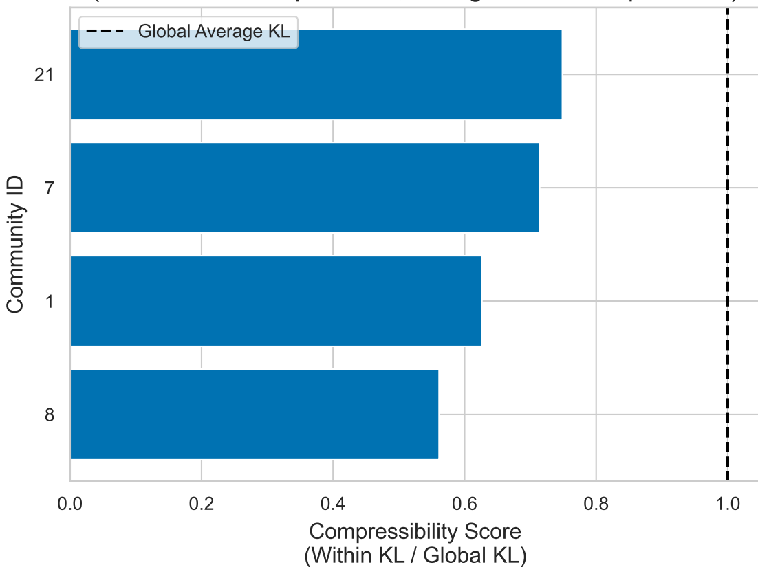
Community Compressibility Ranking — First Layer (Blue = more compressible, Orange = less compressible)
