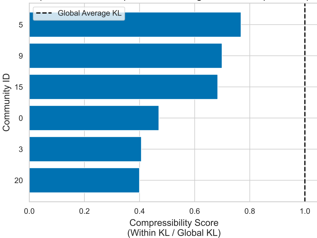
Community Compressibility Ranking — Middle Layer (Blue = more compressible, Orange = less compressible)
