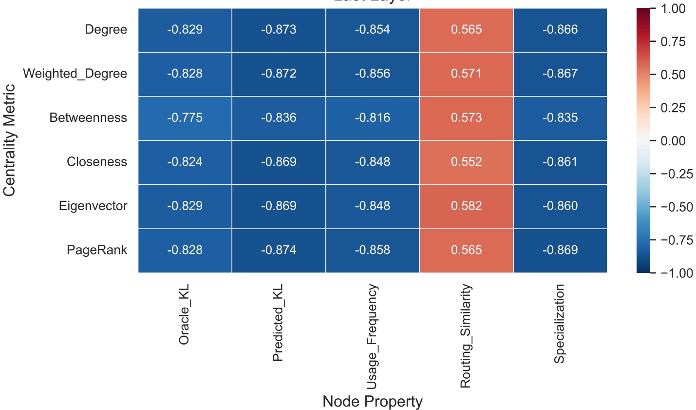
Spearman Correlation: Centrality vs Node Properties Last Layer
