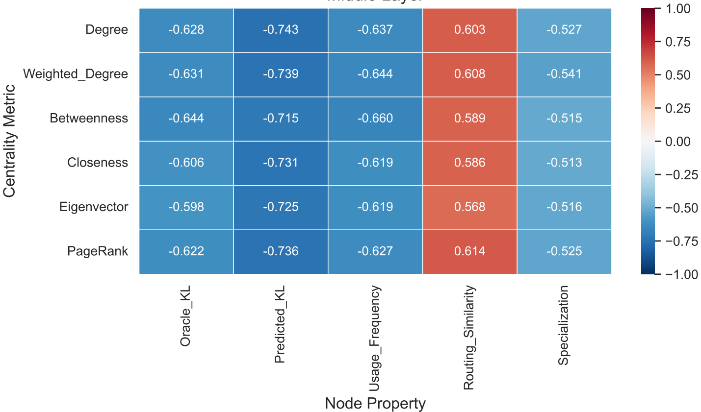
Spearman Correlation: Centrality vs Node Properties Middle Layer
