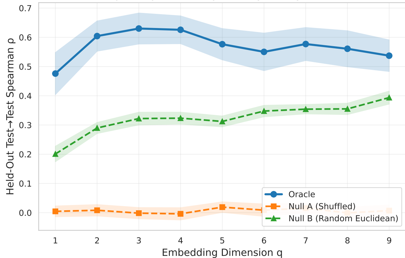
Capability Geometry Fidelity — Layer: first
