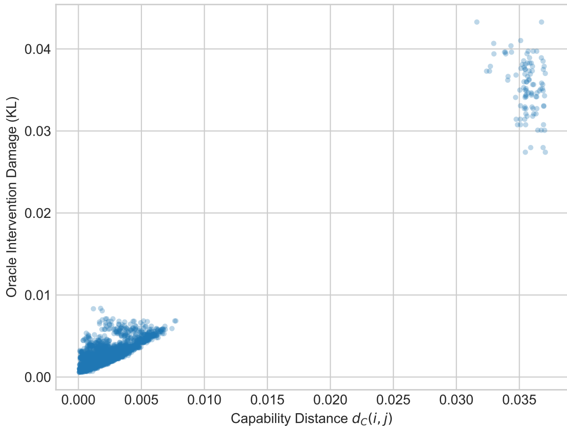
Capability Distance vs Intervention Damage Spearman \rho = 0.7657 (N=3255)
