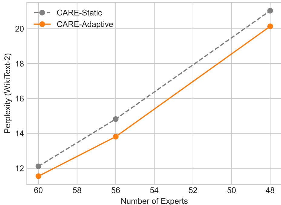
Language Model Quality
