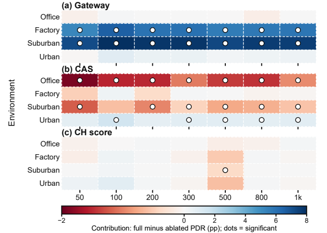
Fig. 4. Expanded NS-3 AERIS ablation across four environments and 50–1000 nodes ( n = 30 per cell). Each heatmap cell reports the full-minus-ablated PDR contribution for one module, environment, and node scale. White circles mark significant full-minus-ablated differences after Welch tests with Holm correction.
