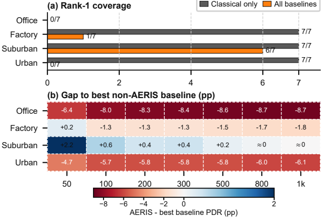
Fig. 2. Expanded NS-3 boundary sweep across four environments and 50–1000 nodes ( n = 30 per cell). Panel (a) reports AERIS rank-1 cells under the classical-only and all-baseline comparisons; panel (b) preserves the full 4-by-7 node-scale grid as the signed PDR gap to the best non-AERIS baseline. Gaps below 0.1 percentage point are near-ties.
