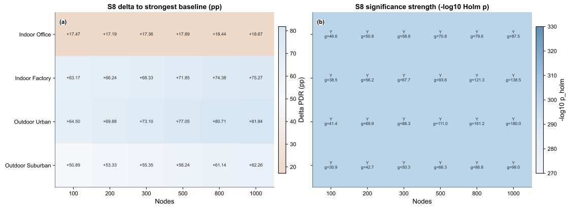
Figure 5. S8 significance map against the strongest baseline per environment-node cell. Panel (a) reports absolute delta (percentage points), and panel (b) reports significance strength as -\log_{10}(p_{\text{Holm}}) with effect-size annotations.
