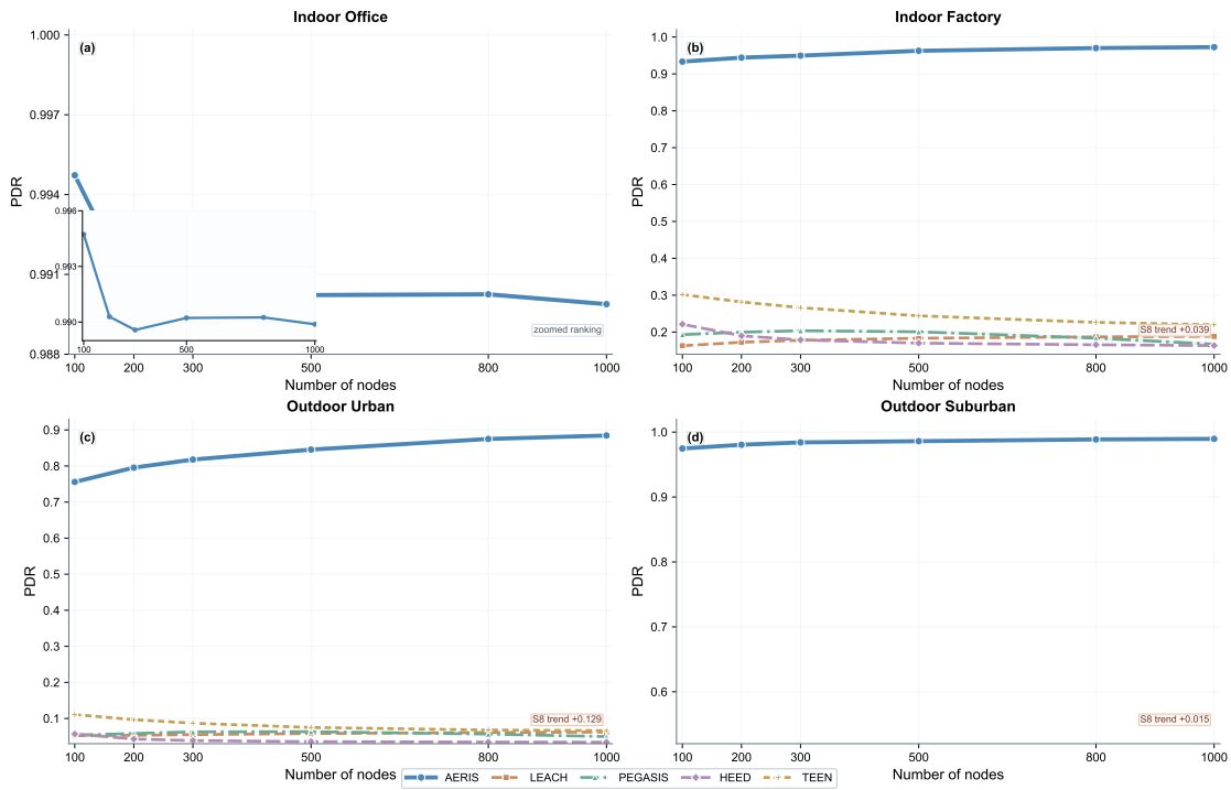
Figure 4. Scalability trends over node counts (balanced n=1000 per environment-node-protocol cell) with 95% CI bands. The indoor_office panel uses a narrowed y-axis window to expose non-zero ordering gaps near PDR=1.0 . Under the original simulator settings (without MAC-collision modeling), AERIS exhibits an increasing trend in three environments; this is treated as a known S8 baseline limitation and is cross-checked with the stricter S9/S10 calibration blocks.
