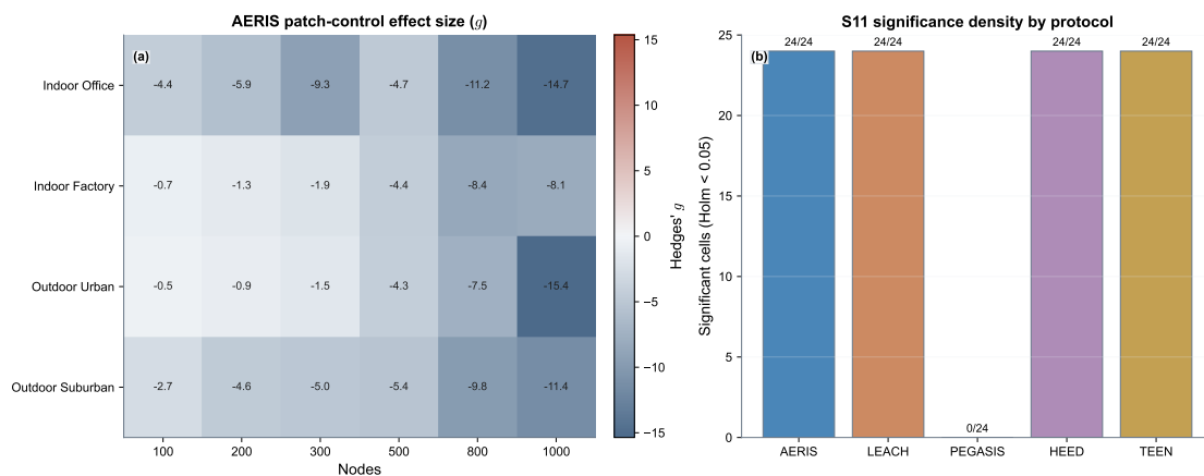
Figure 10. S11 significance density and effect-size map. Panel (a) reports AERIS Hedges' g by environment and node count for patch-control differences. Panel (b) reports the number of Holm-significant cells per protocol (out of 24).
