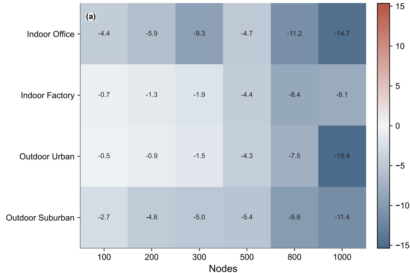
AERIS patch-control effect size ( g )
