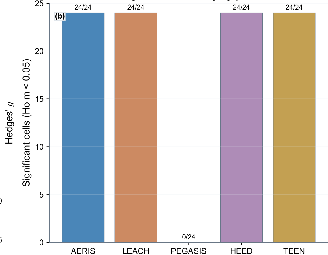
S11 significance density by protocol
