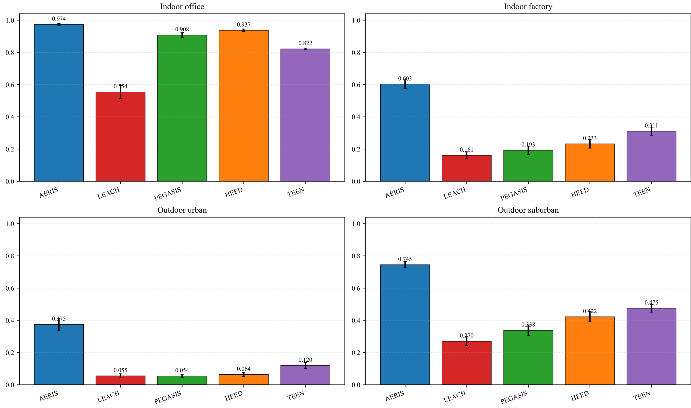
Figure 1. PDR comparison at 100 nodes across four channel environments (n=30)
