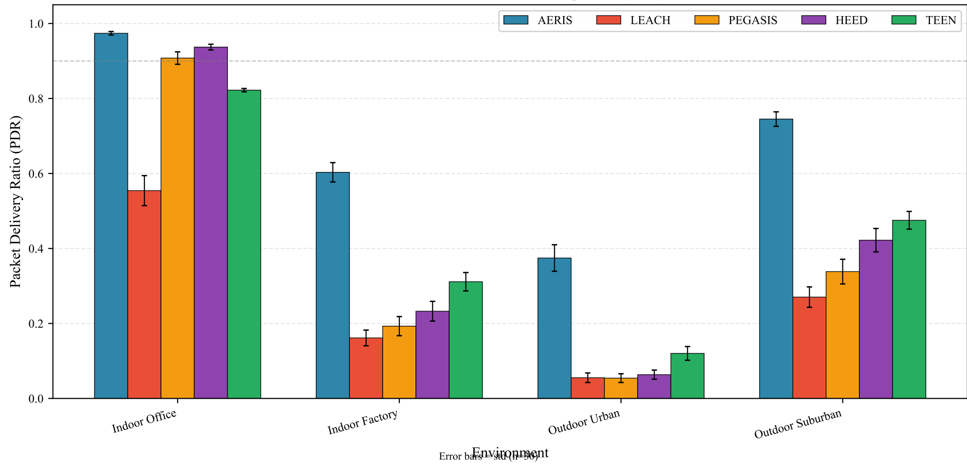
Multi-Environment Protocol Comparison (n=30)
