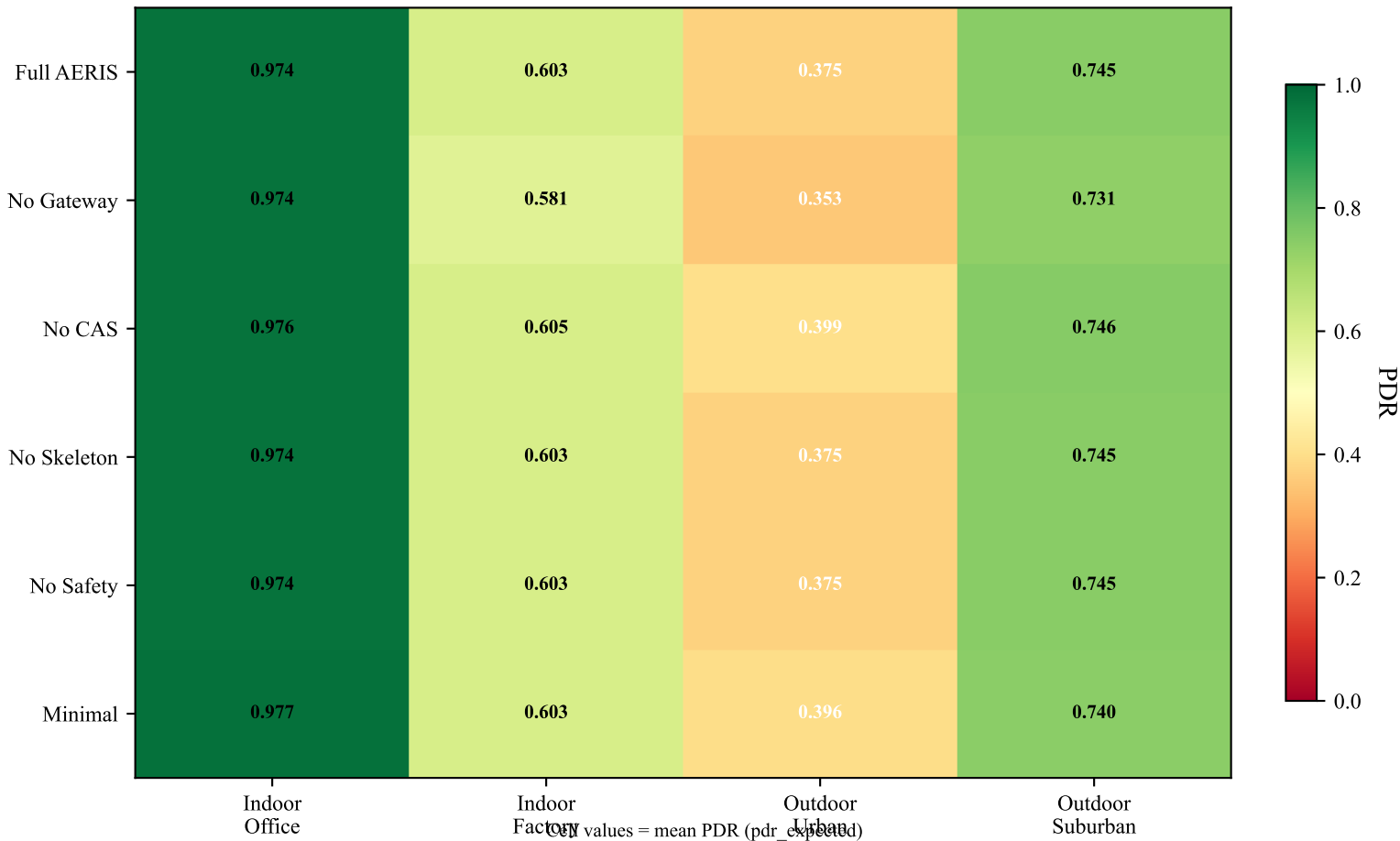
Ablation Study: PDR by Environment and Configuration (n=30)
