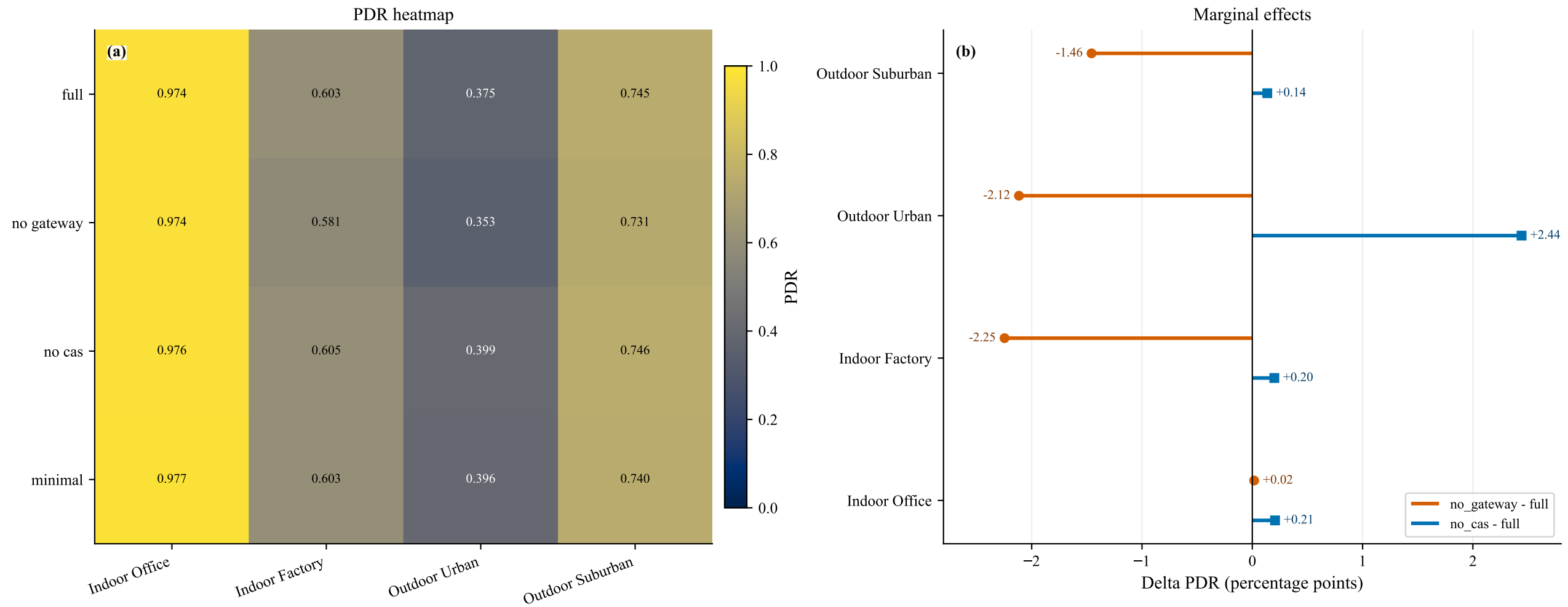
Ablation effects by environment (n=30)
