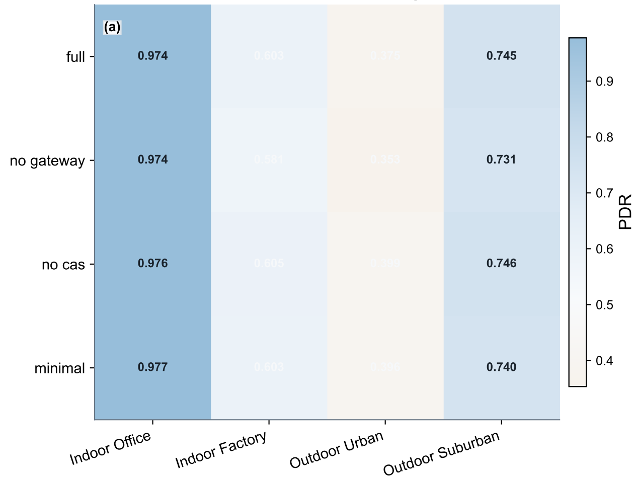
Ablation PDR heatmap
