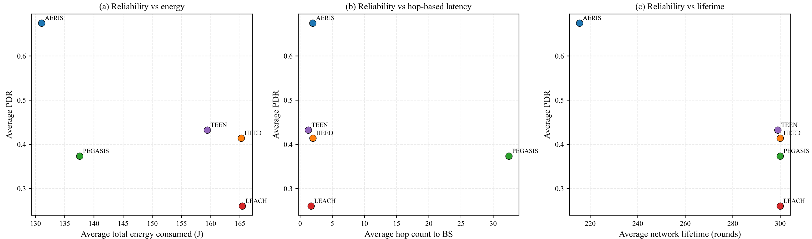
Figure 4. Trade-off summary across protocols (n=30, averaged over 4 environments)
