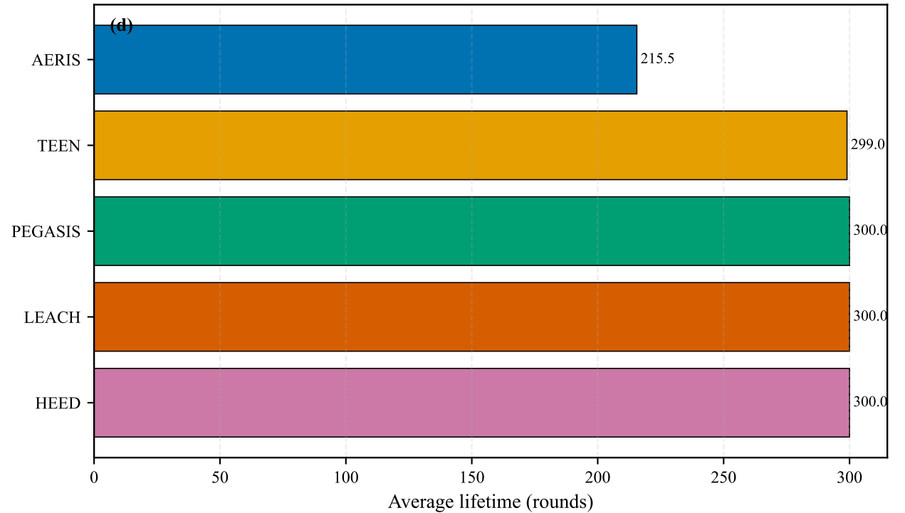
Lifetime ranking
