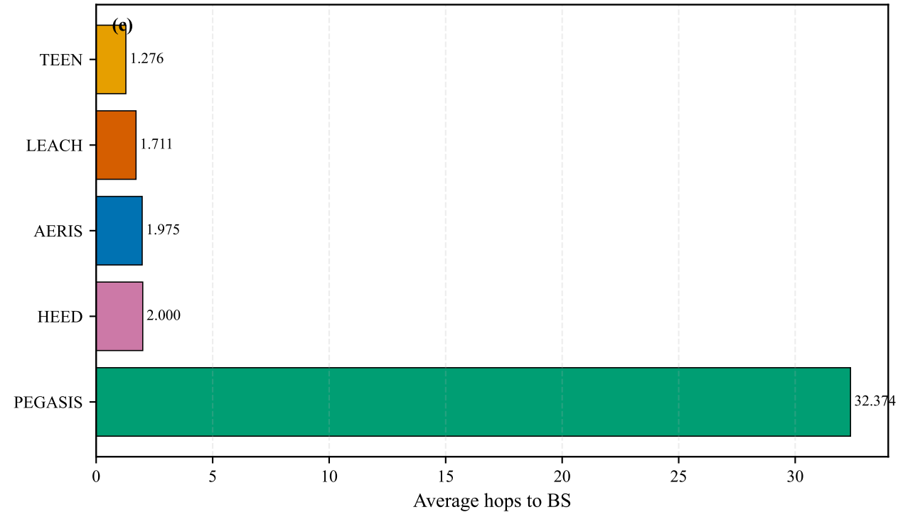
Hop-latency ranking
