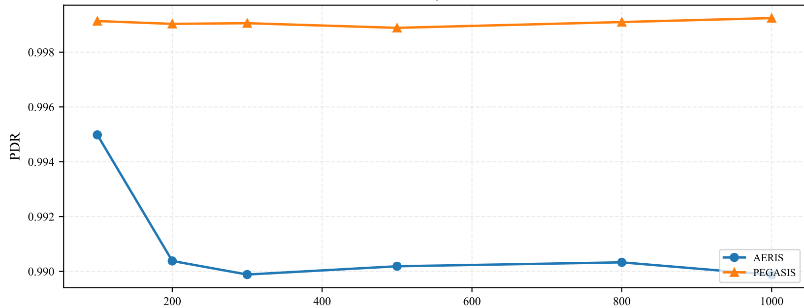
Indoor Office Scalability: AERIS vs PEGASIS
