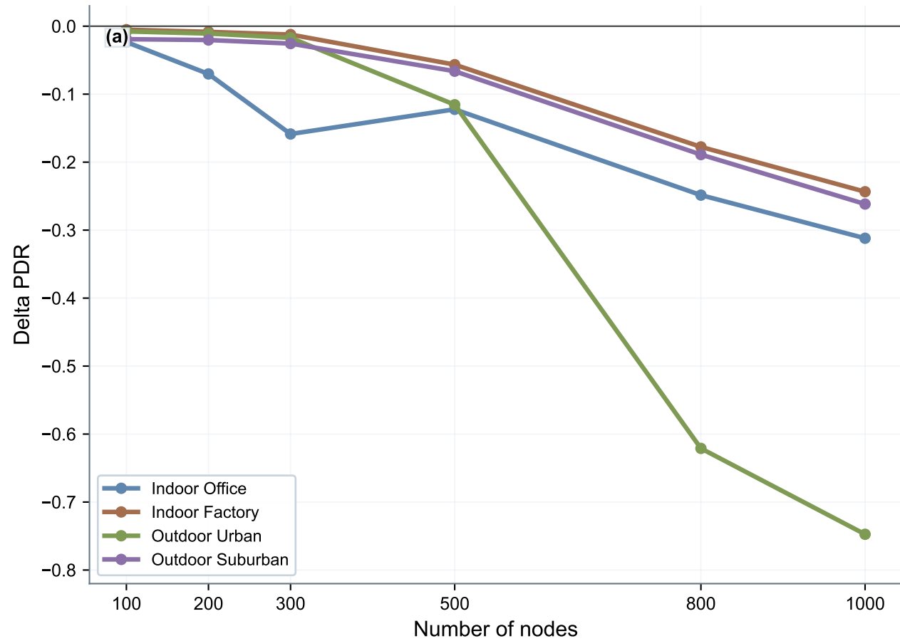
AERIS delta by scale (patch - control)
