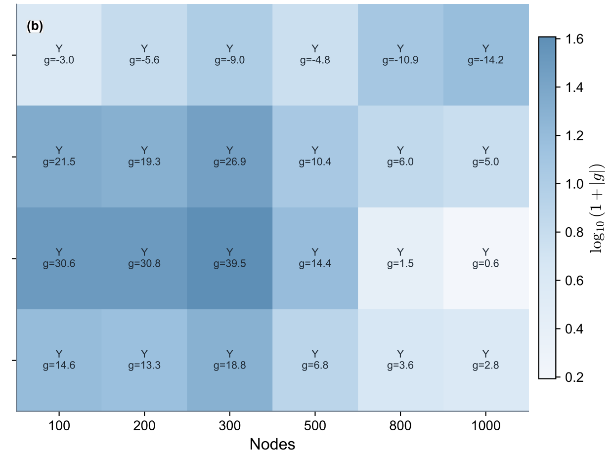
v50-rigor significance strength
