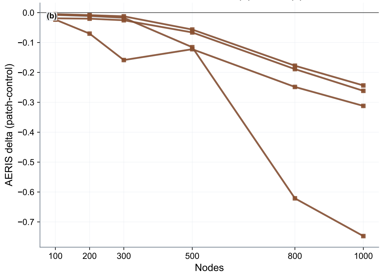
AERIS stress deltas: S9 (o) vs S11 (s)
