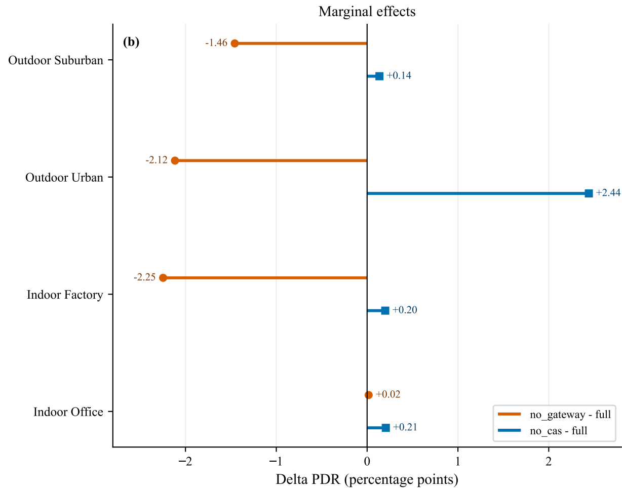
Ablation effects by environment (n=30)
