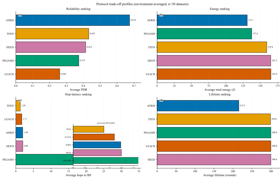
Figure 4. Trade-off panel from publication-tier data: reliability, energy, hop-based latency, and lifetime. The hop panel includes a local zoom to resolve non-PEGASIS protocols under a highly skewed hop scale.
