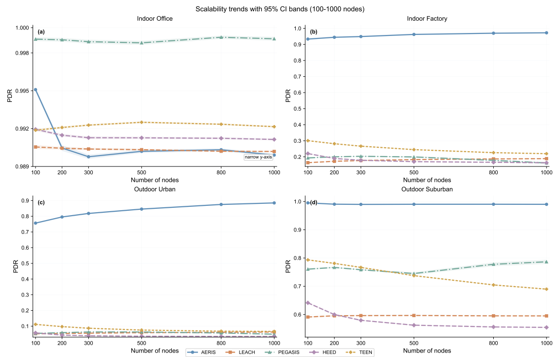
Figure 3. Scalability trends over node counts (indoor_factory n=650 , other environments n=550 ) with 95% CI bands. The indoor_office panel uses a narrowed y-axis window to expose small but non-zero ordering gaps near PDR=1.0 .
