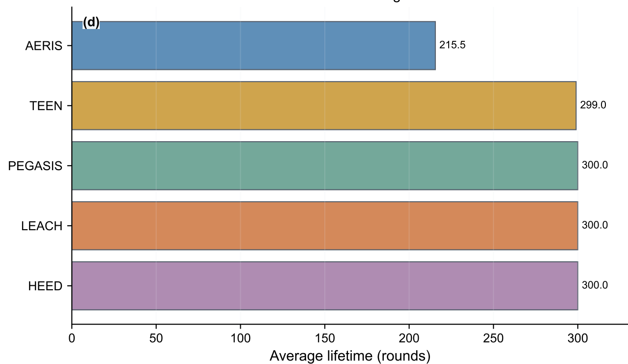
Lifetime ranking
