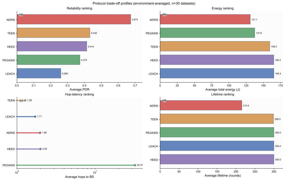
Figure 4. Trade-off panel from publication-tier data: reliability, energy, hop-based latency, and lifetime. The hop panel uses a logarithmic x-axis to keep low-hop and high-hop protocols visible in the same frame without overlap.
