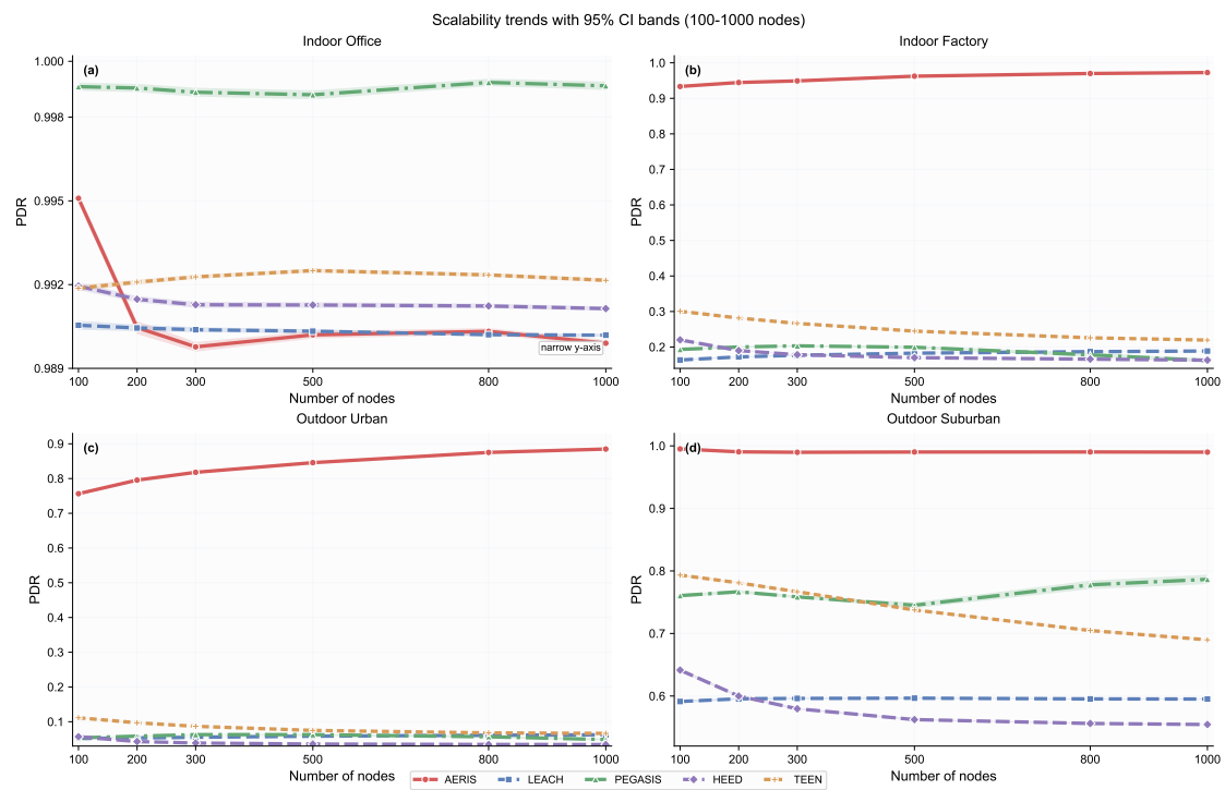
Figure 3. Scalability trends over node counts (indoor_factory n=650 ; indoor_office, outdoor_urban, and outdoor_suburban n=550 ) with 95% CI bands. The indoor_office panel uses a narrowed y-axis window to expose non-zero ordering gaps near PDR=1.0 .
