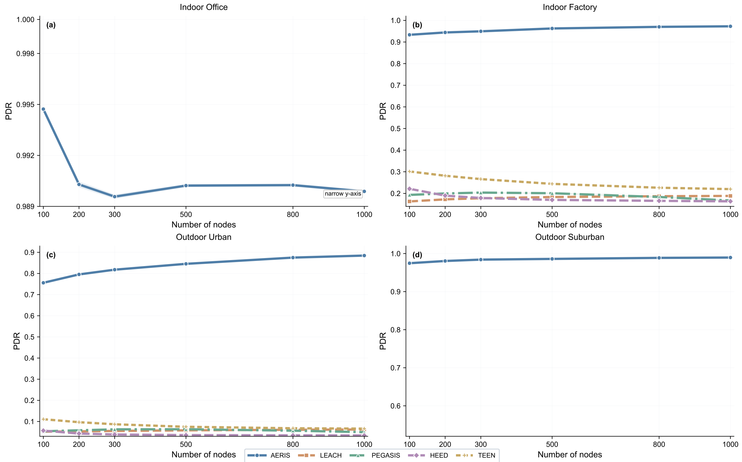
Scalability trends with 95% CI bands (100-1000 nodes)
